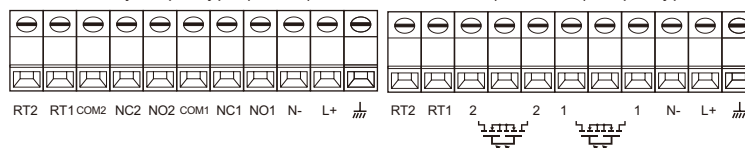
Relay output type (DPDT)
