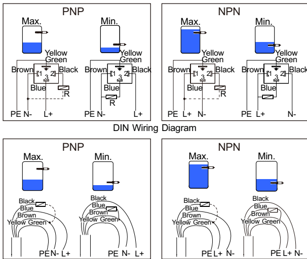
M12x1 Cable Wiring Diagram
