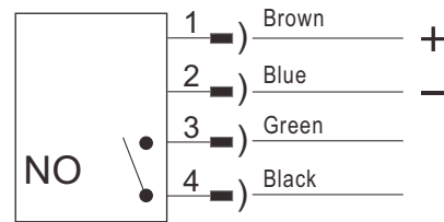
Fig. 10, Relay output type wiring (NO)
