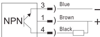
Fig. 7, NPN output type wiring
